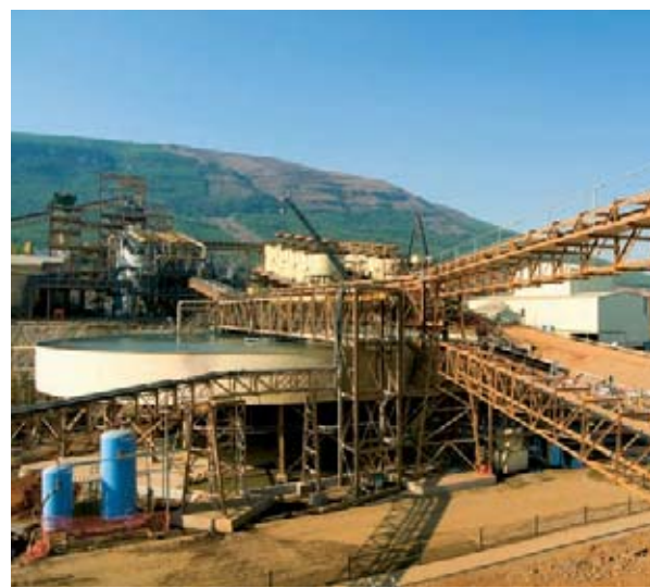
Nkomati PCMZ plant tailings thickener
