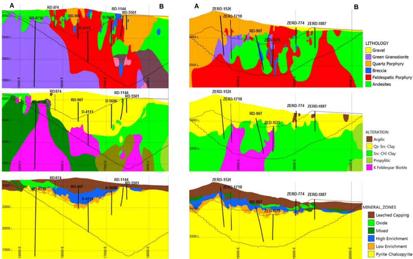
Figure 4: Escondida (left) and Escondida Norte (right) geological sections. Geology (upper row), alteration (middle row) and mineral zones (lower row).
