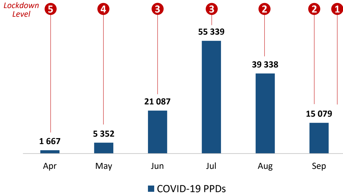
COVID-19 PPDs
